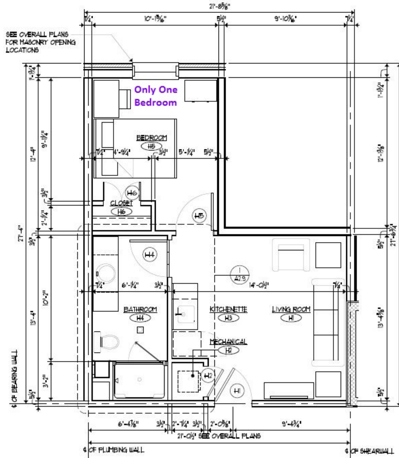
3 SUITE 'H' PLAN A2.7 1/4" = 1'-0" (FIRST FLOOR ONLY)
