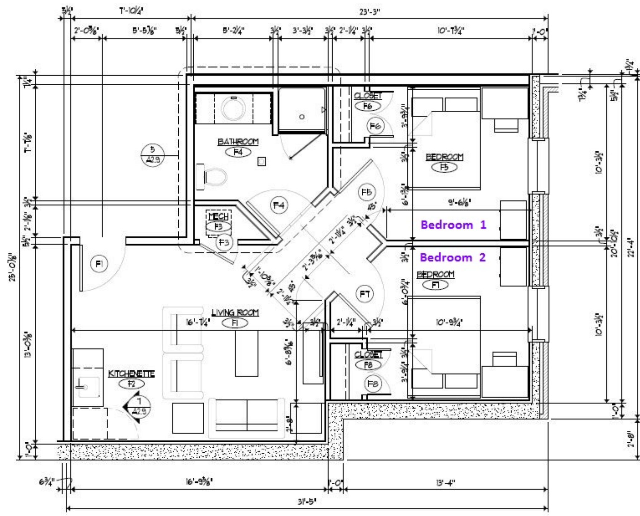
2 SUITE 'F' PLAN A2.1 1/4" = 1'-0" (FIRST FLOOR ONLY)
