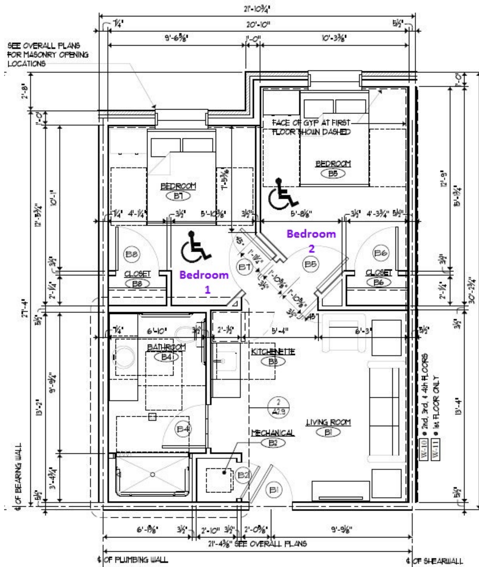
2 SUITE 'B' PLAN A2.6 1/4" = 1'-0" ACCESSIBLE
